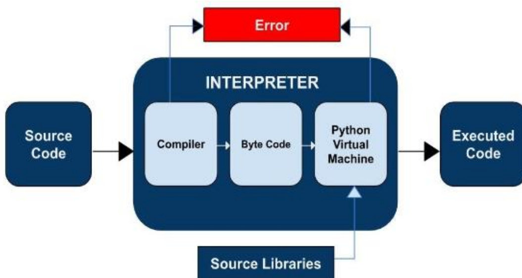
Figure 2.1: Python Execution Architecture
